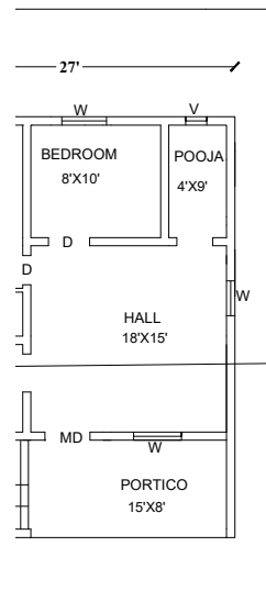
PROPOSED GROUND FLOOR
