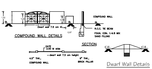
FOUNDATION DETAILS SCALE : 1:50
