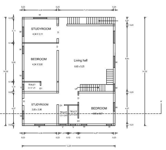
PRO. FIRST FLOOR PLAN
