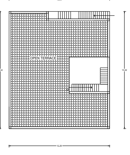
TERRACE PLAN
