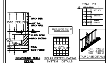
AREA DETAIL
