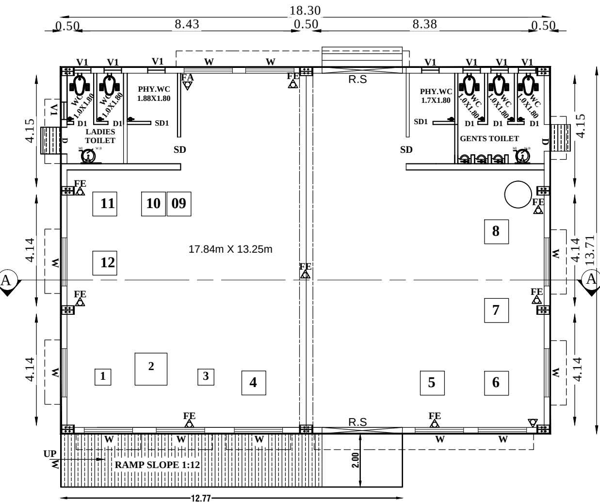
MAIN BUILDING (BLOCK-1) GROUND FLOOR PLAN
