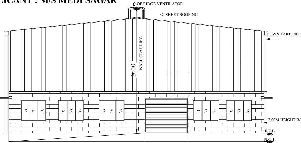
ELEVATION- SOUTH FACING (BLOCK-1)
