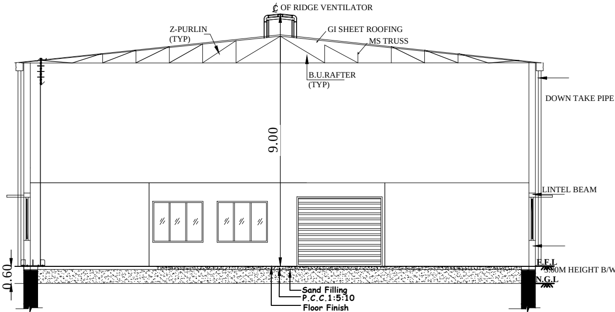
SECTION - AA ( BLOCK 1)
