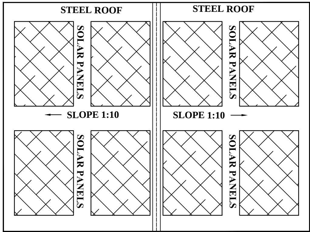
MAIN BUILDING (BLOCK-1) ROOF PLAN
