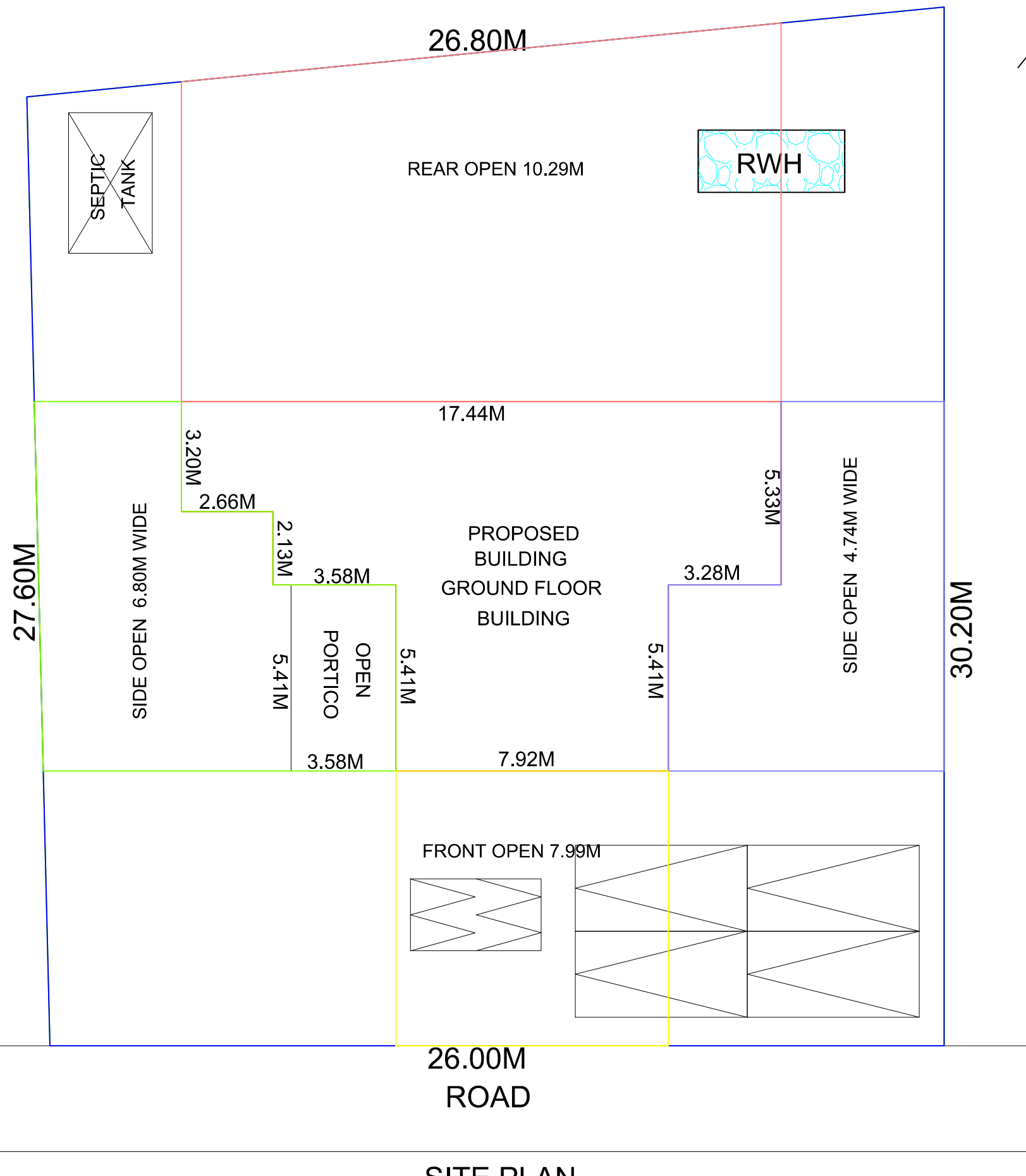
SITE PLAN
