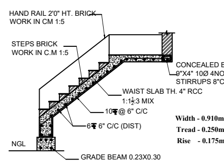
STAIRCASE DETAILS (Scale 1:50)
