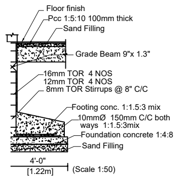
FOUNDATION DETAILS
