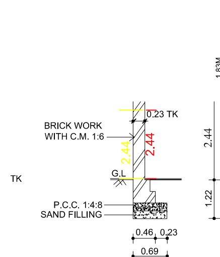
SECTION OF COMPOUND WALL
