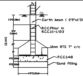
FOUNDATION DETAILS
