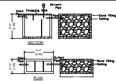
DETAILS OF SEPTIC TANK & DISPERSION TRENCH
