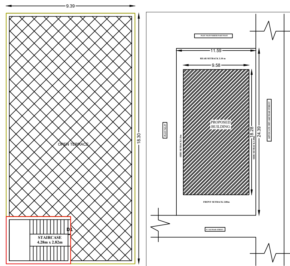
PROPOSED TERRACE FLOOR
