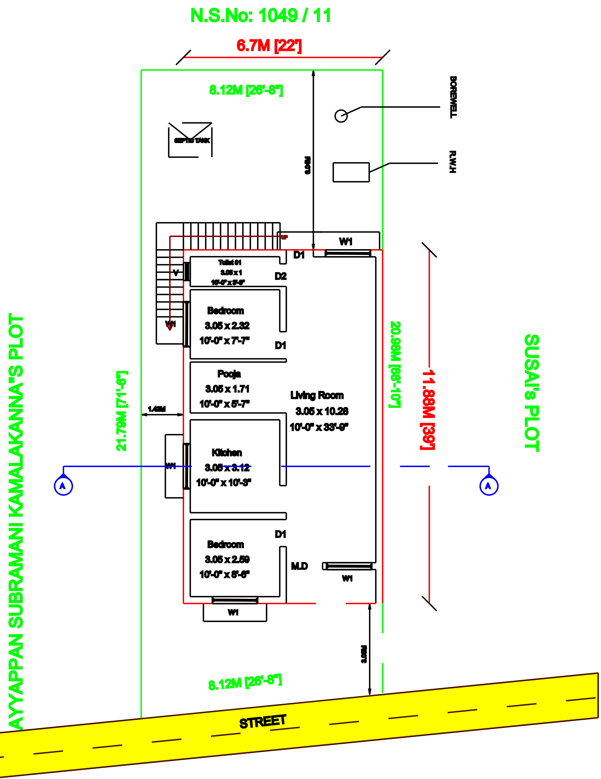
M GROUND FLOOR PLAN
