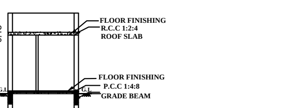
SECTION - BB' (BLOCK-1)
