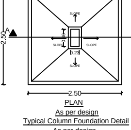
Typical Column Foundation Detail
