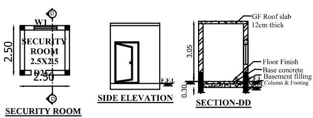
SECURITY ROOM PLAN
