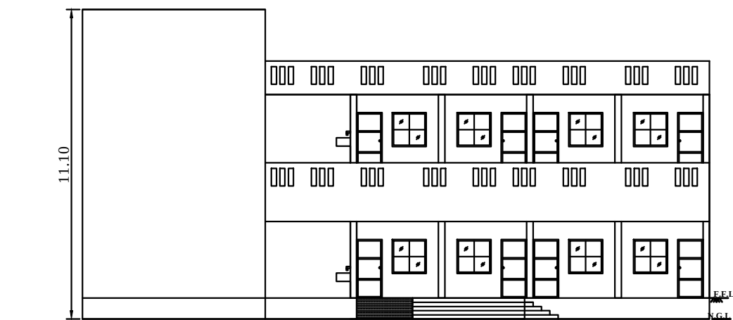
ELEVATION (BLOCK-1)
