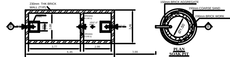
PLAN SEPTIC TANK
