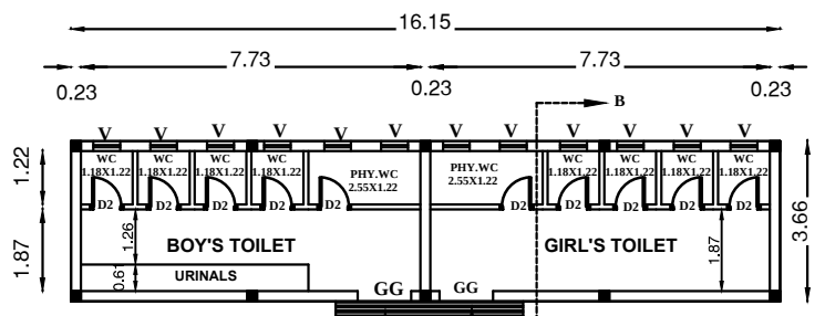
GROUND FLOOR TOILET PLAN (BLOCK-2)
