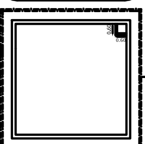
REINFORCEMENT DETAIL FOR SUMP UNDER GROUND RAW WATER SEWAGE SUMP CAPACITY - 108 M 3
