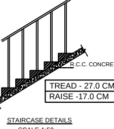
STAIRCASE DETAILS SCALE:1:50
