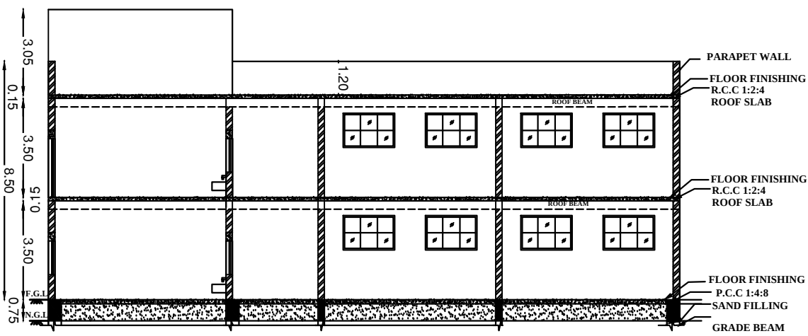
SECTION - AA' (BLOCK-1)
