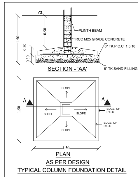
TYPICAL COLUMN FOUNDATION DETAIL
