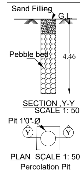
SECTION Y-Y SCALE 1: 50
