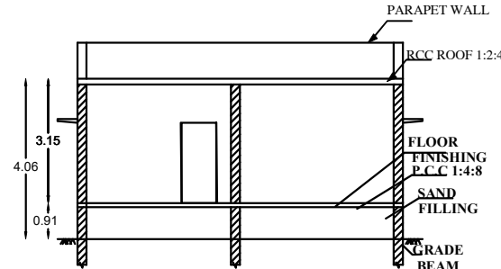
SECTION
