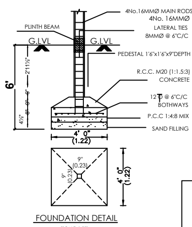
FOUNDATION DETAIL
