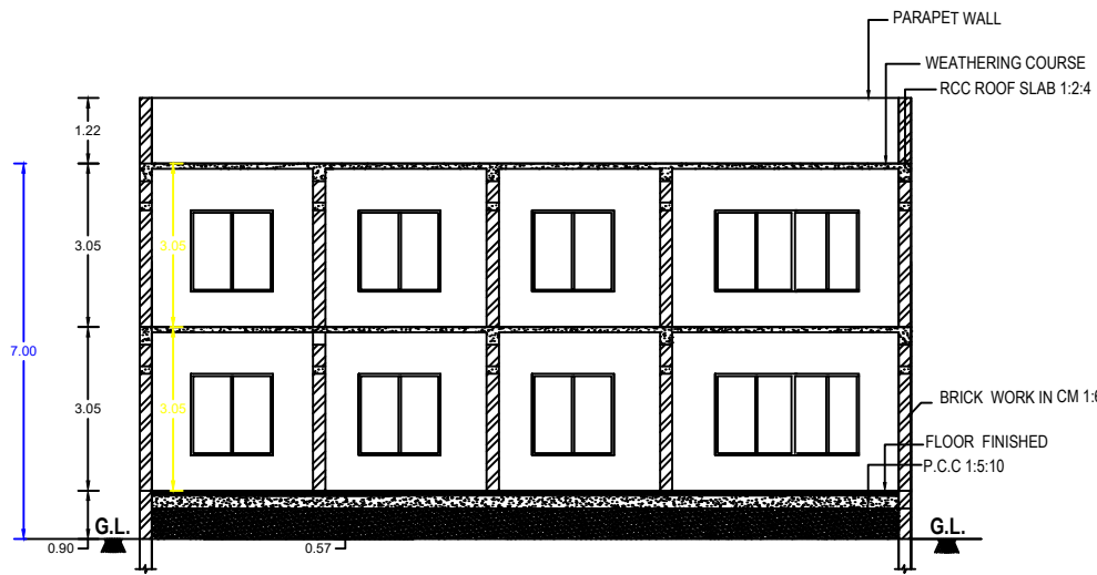
SECTION "A-B"
