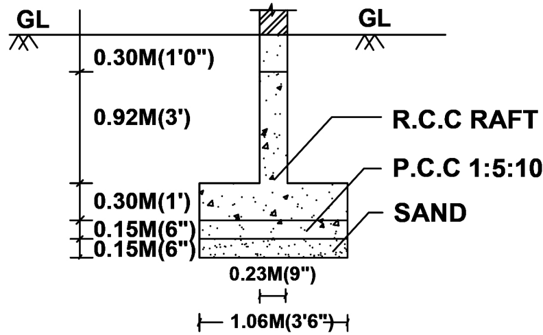
"FOUNDATION DETAILS"
