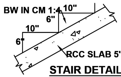
STAIR DETAIL
