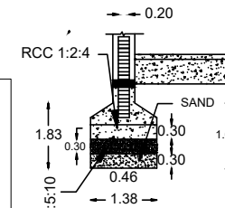
SECTION Z-Z
