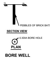
BORE WELL
