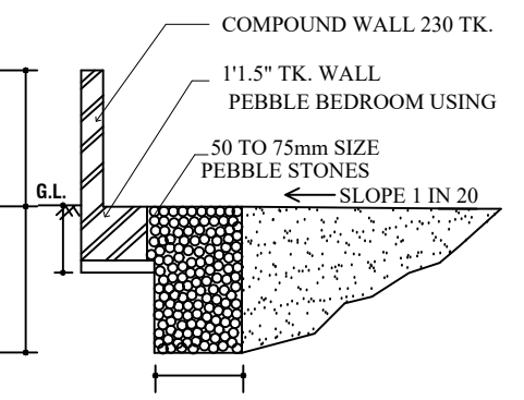
RAIN WATER COLLECTION TRENCH (SCALE-1:100)
