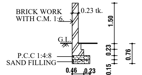
SECTION OF COMPOUND WALL
