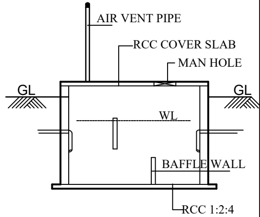
SECTIONAL ELEVATION SEPTIC TANK
