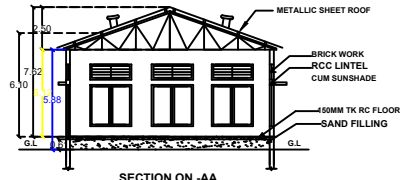
SECTION ON-AA
