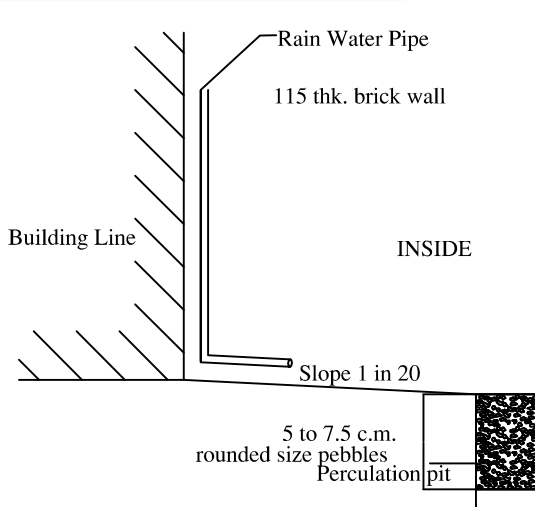
PERCOLATION PIT
