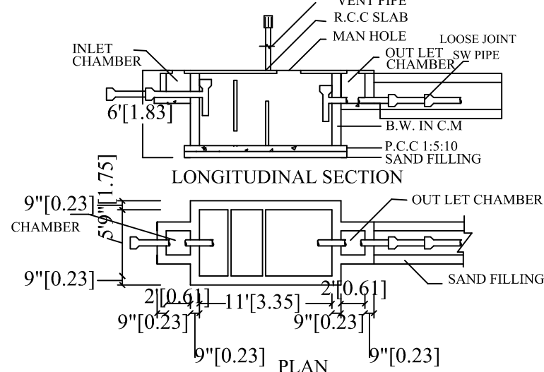
SEPTIC TANK:
