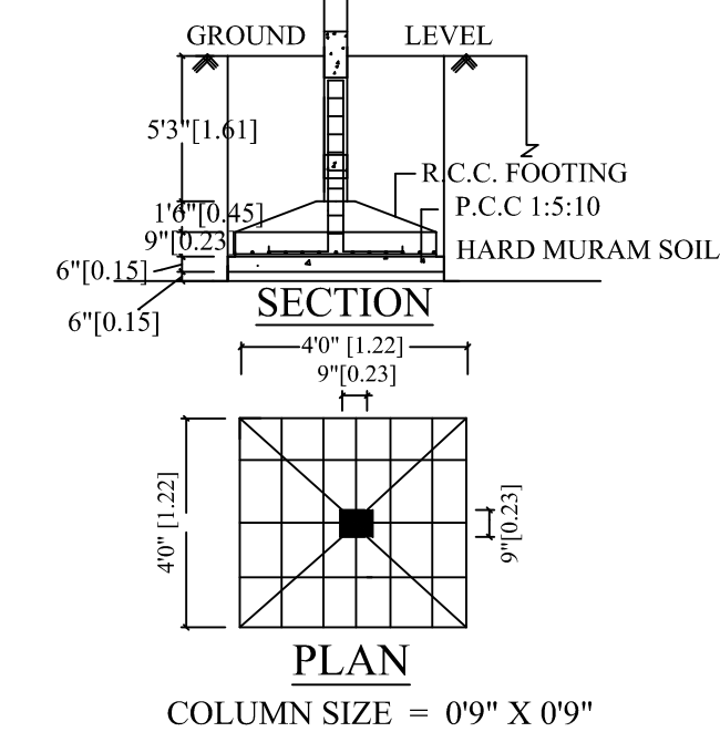
FOUNDATION DETAILS
