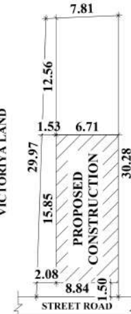
SITE PLAN
