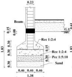
SECTION Z-Z
