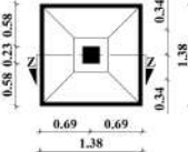
COLUMN FOOTING
