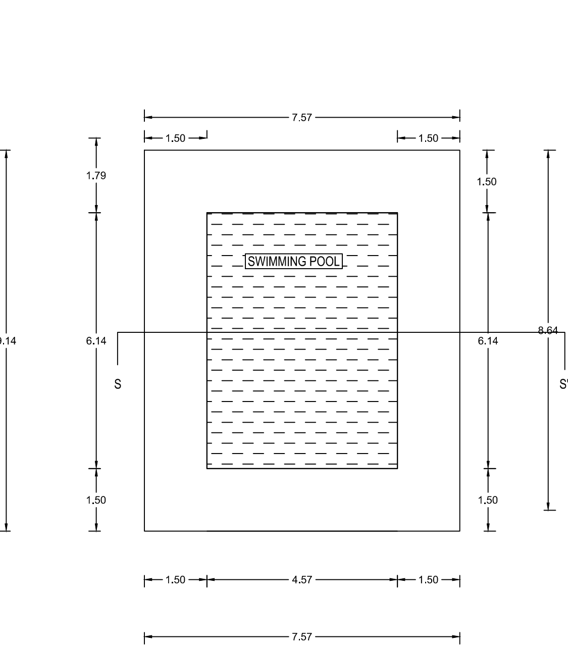
SWIMMING POOL
