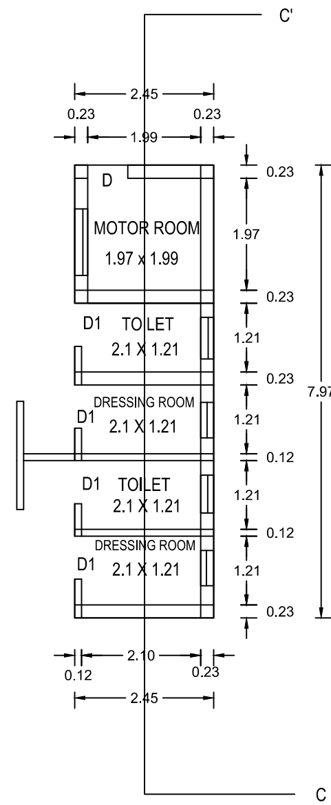
TOILET BLOCK
