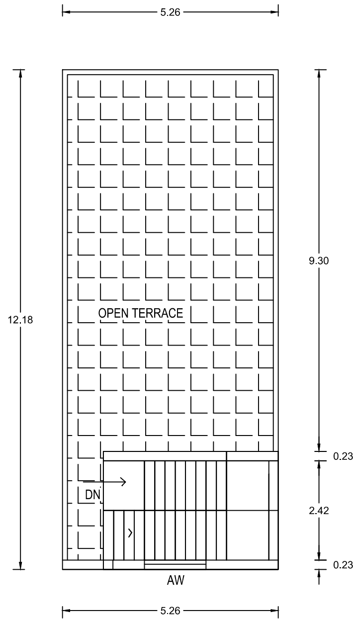
TERRACE
