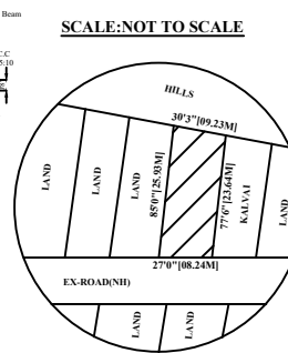
TOPO PLAN..
