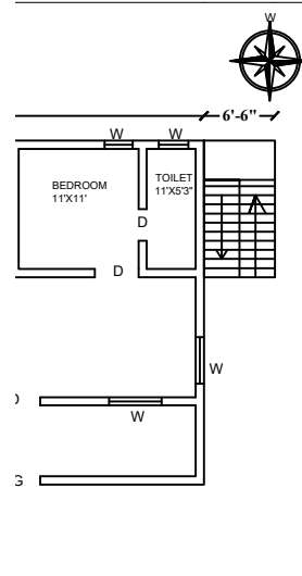
PROPOSED GROUND FLOOR
