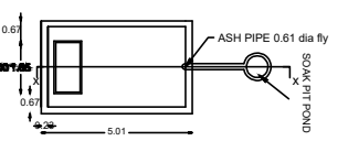
DETAIL OF SEPTIC TANK
