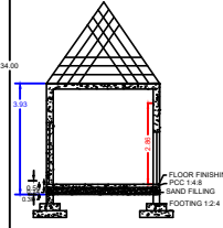
BLOCK - 2 SECTION
