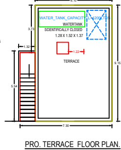
PRO. TERRACE FLOOR PLAN.
