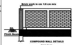
COMPOUND WALL DETAILS
