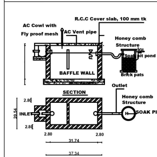
PLAN SEPTIC TANK
