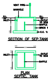
RAIN WATER HARVESTING SYSTEM RWH_CAPACITY_L=1000LTRS
