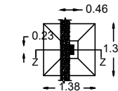
COLUMN FOOTING DETAIL
