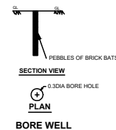
BORE WELL
