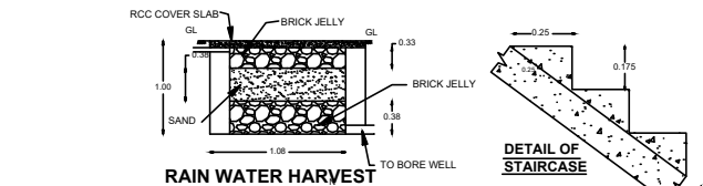
RAIN WATER HARVEST
