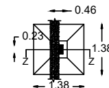
COLUMN FOOTING DETAIL
