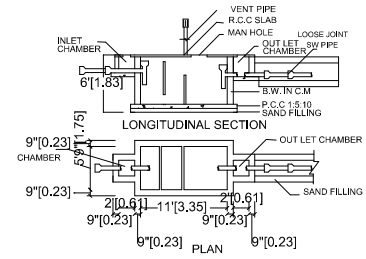
SEPTIC TANK:
