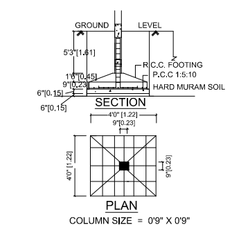
FOUNDATION DETAILS
