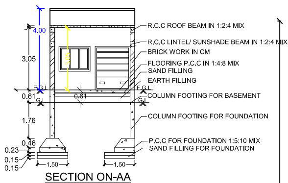
SECTION ON-AA
