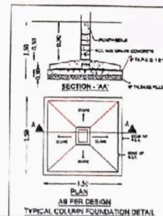
AS PER DESIGN TYPICAL COLUMN FOUNDATION DETAIL
