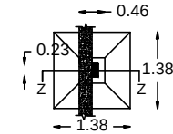
COLUMN FOOTING DETAIL
