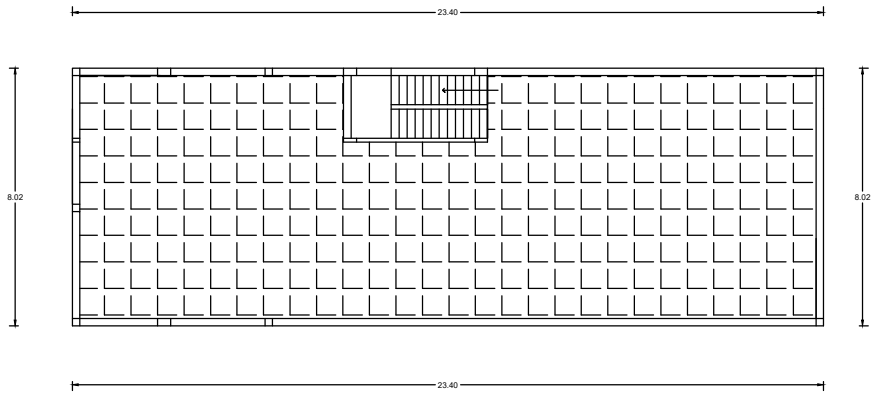
TERRACE PLAN
