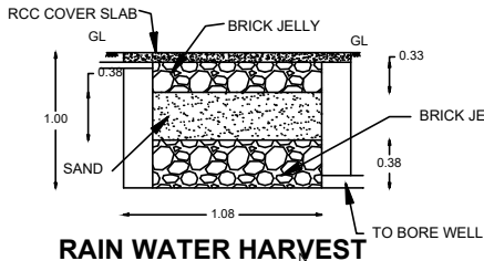
RAIN WATER HARVEST
