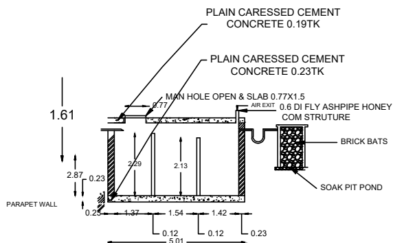
SECTION XX
