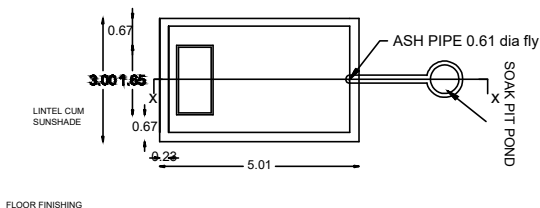
DETAIL OF SEPTIC TANK
