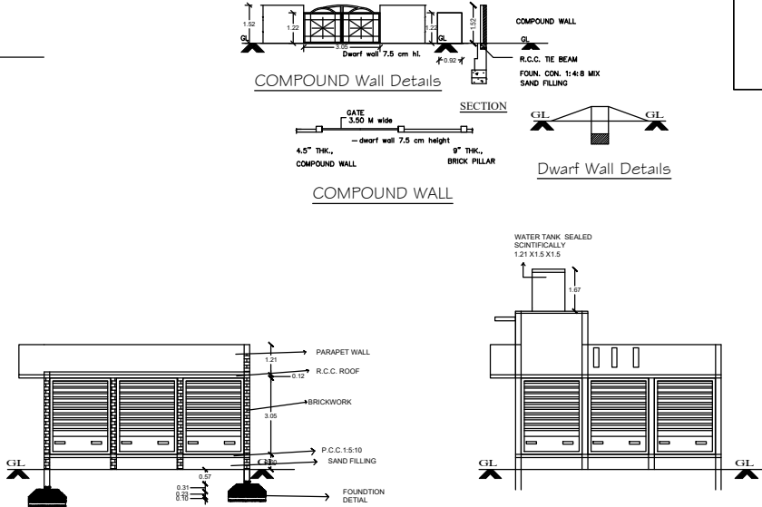
SECTION-AA'
