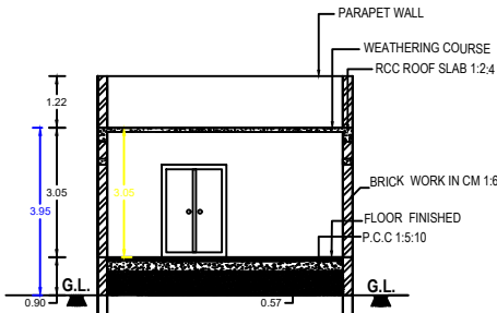
SECTION "A-B"
