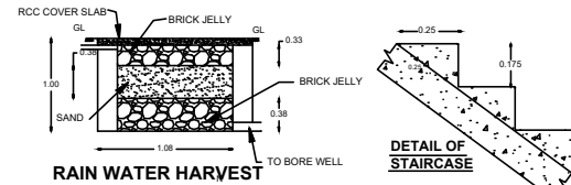
RAIN WATER HARVEST
