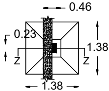
COLUMN FOOTING DETAIL
