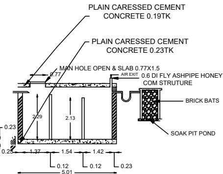
SECTION XX
