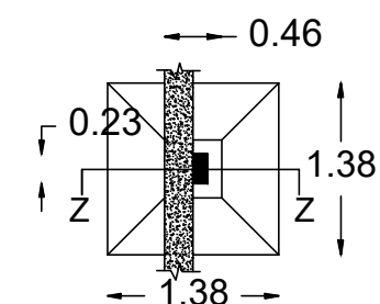
COLUMN FOOTING DETAIL
