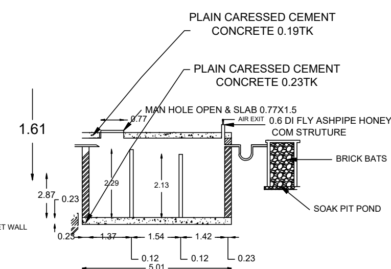
SECTION XX
