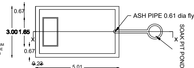
DETAIL OF SEPTIC TANK
