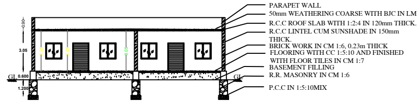
SECTION ON AB
