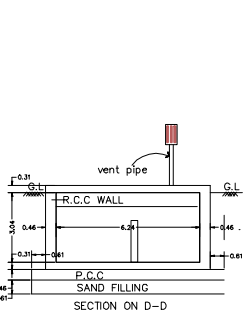
SECTION ON D-D
