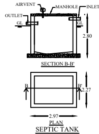
SEPTIC TANK
