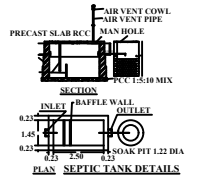
PLAN SEPTIC TANK DETAILS
