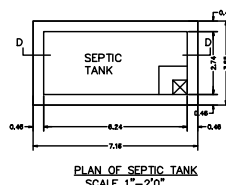
PLAN OF SEPTIC TANK SCALE 1\"/>
