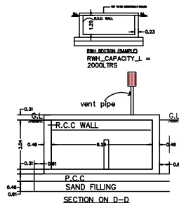
SECTION ON D-D
