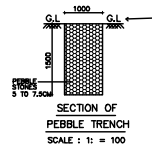
SECTION OF PEBBLE TRENCH SCALE : 1: = 100
