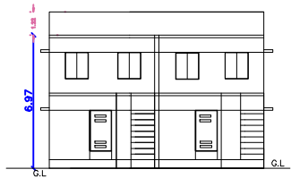
FRONT ELEVATION
