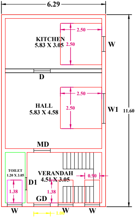
PLAN AT GROUND FLOOR
