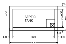
PLAN OF SEPTIC TANK SCALE: 1" = 2'-0"
