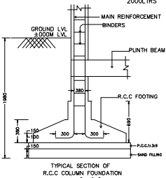
TYPICAL SECTION OF R.C.C. COLUMN FOUNDATION SCALE: 1" = 2'-0"
