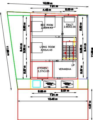
EXISTING GROUND FLOOR PLAN
