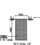
SECTION OF PEBBLE TRENCH SCALE: 1" = 10'
