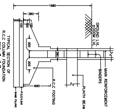
TYPICAL SECTION OF R.C.C. COLUMN FOUNDATION
