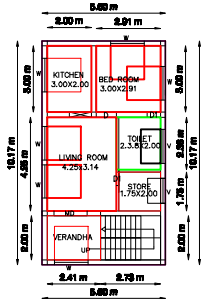
PRO.FIRST FLOOR PLAN
