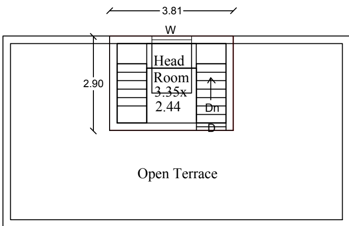
HEAD ROOM PLAN
